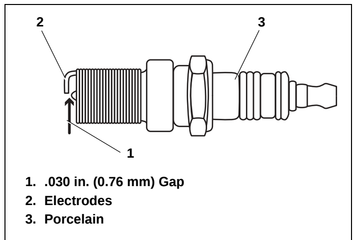
Figure 23. Spark Plug
