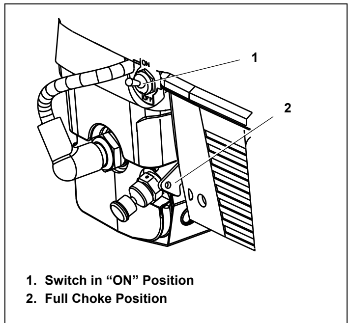
Figure 11. Switch and Full Choke Positions
