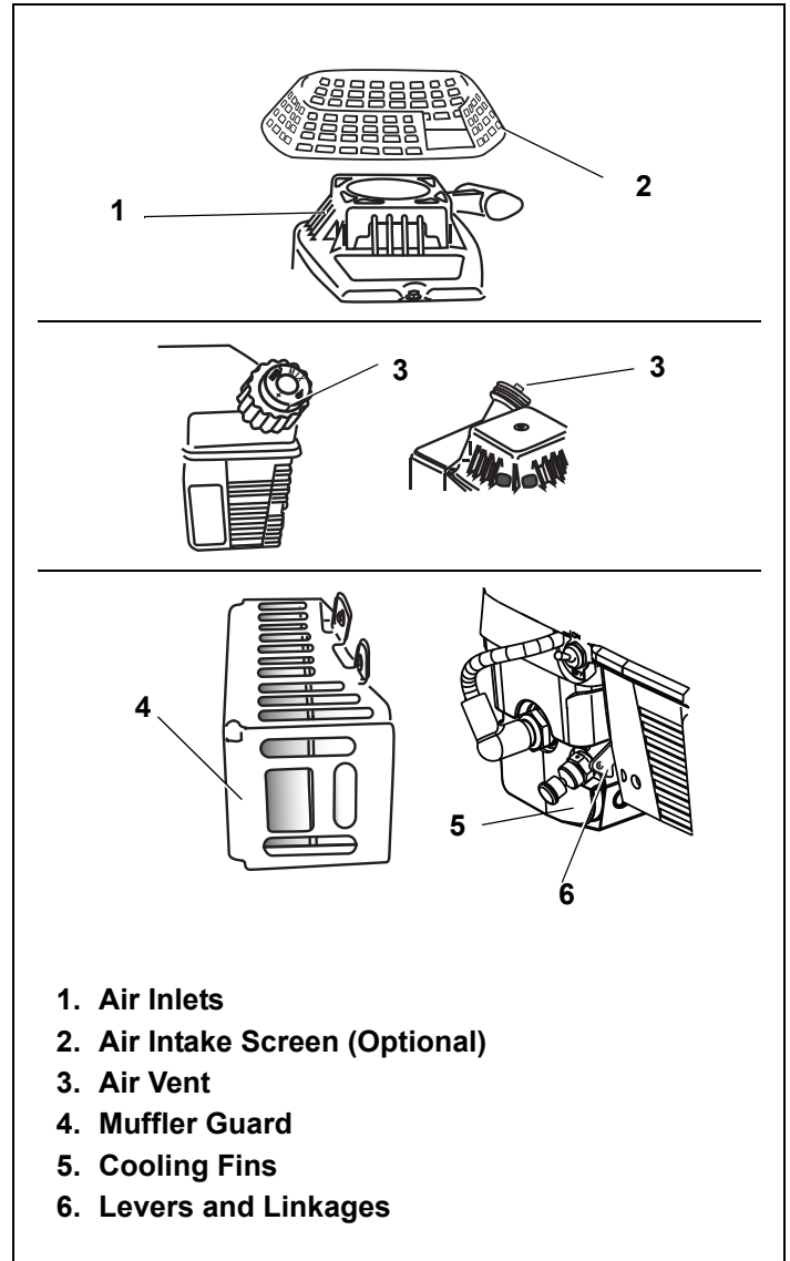
Figure 19. Debris Removal Areas
